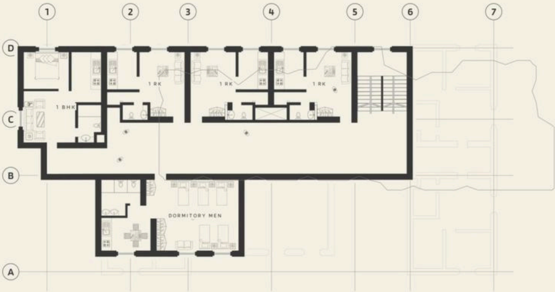
FIRST FLOOR RL 102.80 · +3.80
