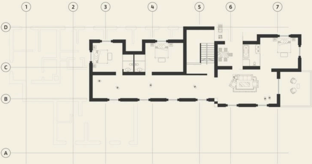
SECOND FLOOR RL 105.80 · +6.80
