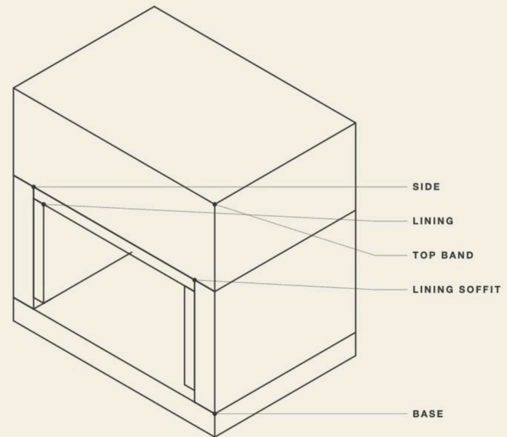
ISOMETRIC
