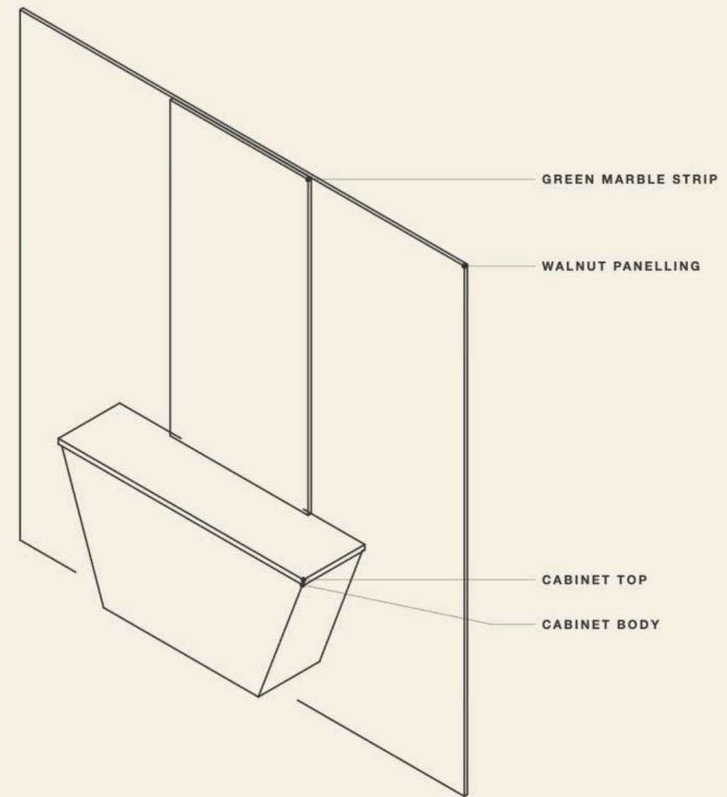
ISOMETRIC
