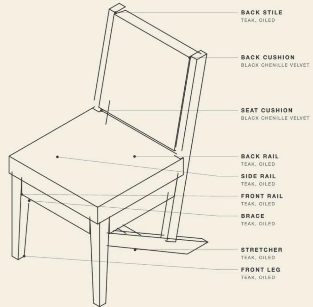
ISOMETRIC
